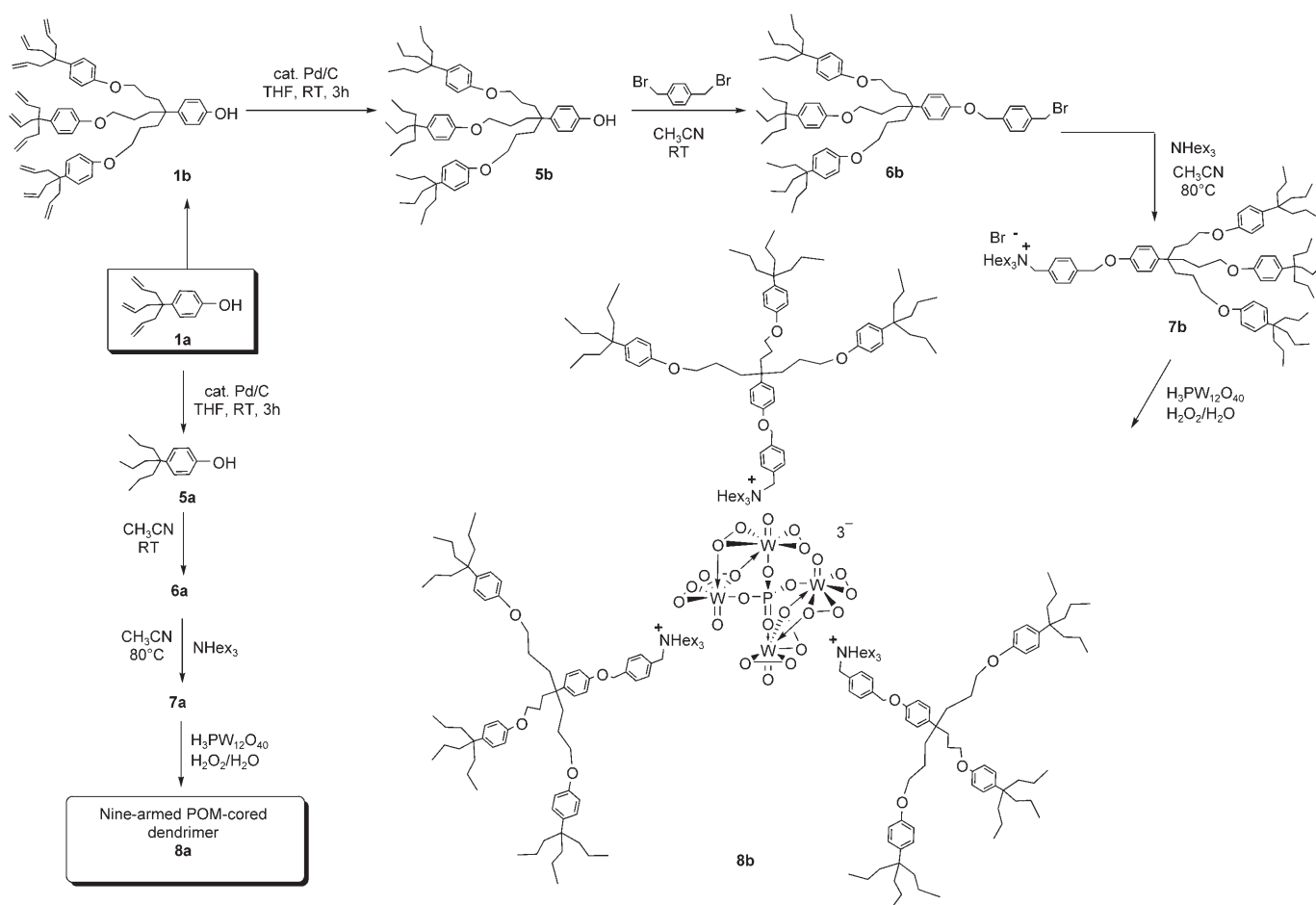
Scheme 2. Syntheses of the n -propyl-terminated 9- and 27-armed POM-cored dendrimers 8a and 8b .
