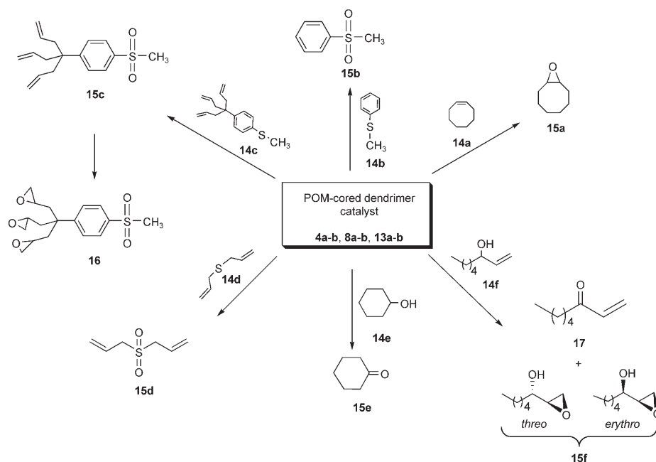
Scheme 4. Catalytic oxidation reactions with 0.4 mol% of 9- and 27-armed POM-cored dendrimers 4a, b , 8a, b , and 13a, b , substrate (250 equiv), \text{H}_2\text{O}_2 (800 equiv), and \text{CDCl}_3 (3 mL).
